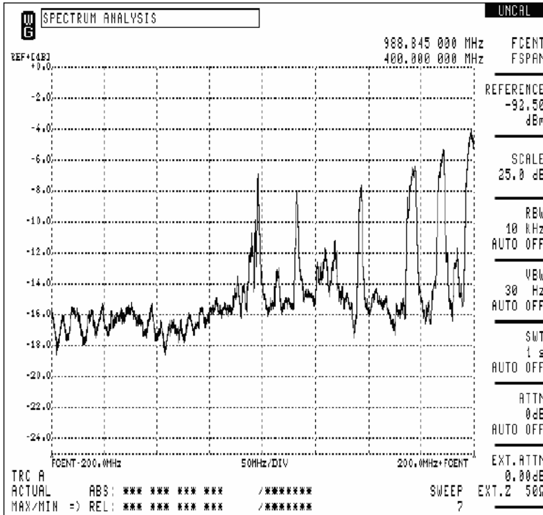
Fig. 4 Spectrum of the 332.5 °E sat. with 400 MHz Span
