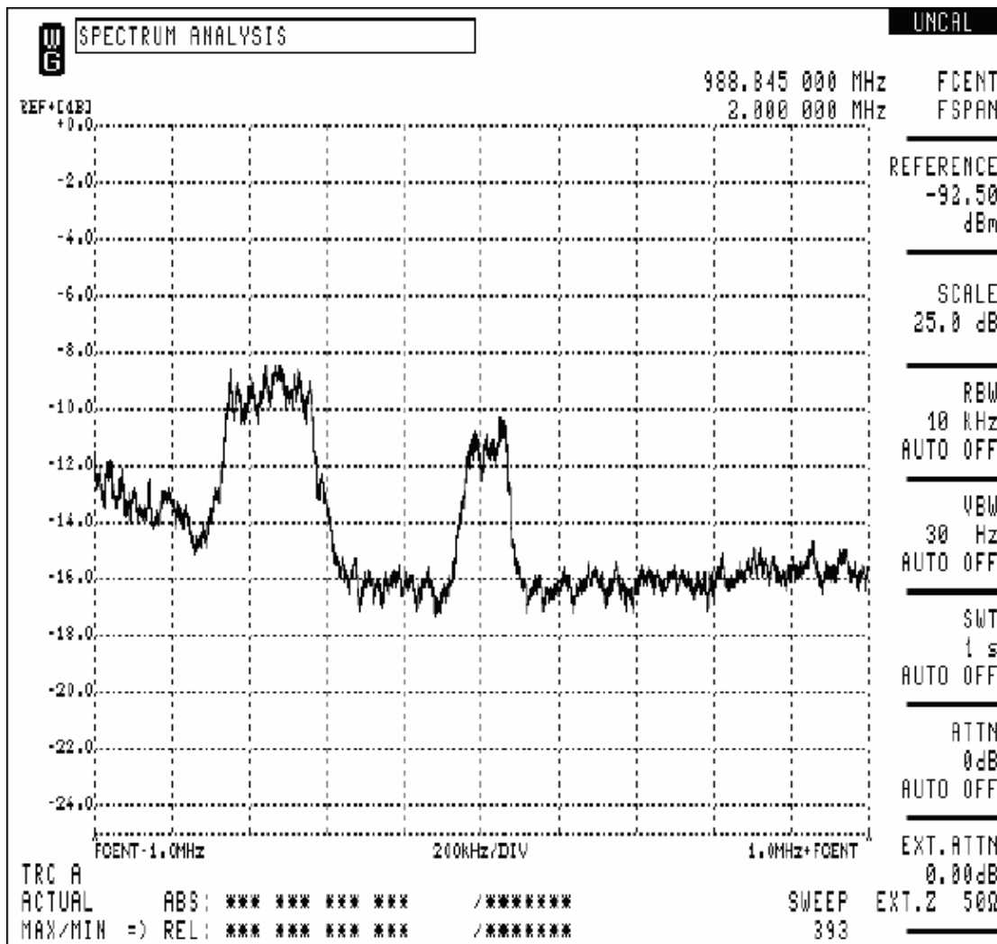
Fig. 2 Spectrum of the 332.5 °E sat. with 2 MHz Span
