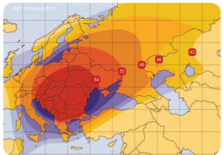
AMOS 2 @ 4° W typical KU band downlink coverage
